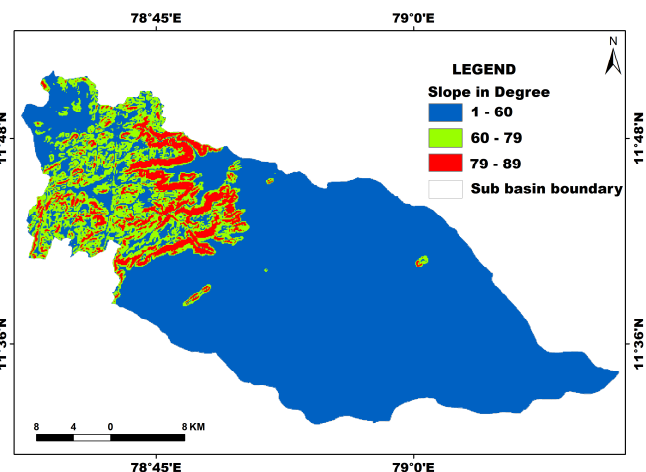
Fig. 4 Slope map
