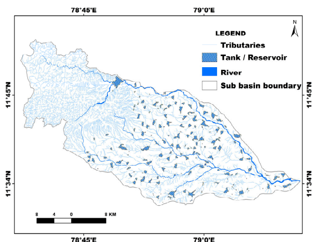
Fig. 3 Drainage map
