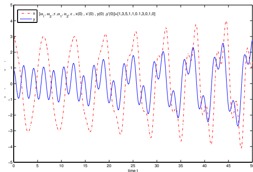
Fig. 1. Plots of x = x_0 + x_1 and y = y_0 + y_1 for [\omega_1, \omega_2, \tau, \alpha_1, \alpha_2, \varepsilon, x(0), \dot{x}(0), y(0), \dot{y}(0)] = [1, 3, 5, 1, 1, 0.1, 3, 0, 1, 0] .
