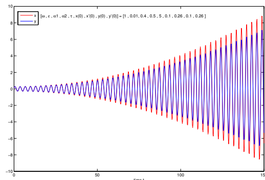
Fig. 3. Plots of x = x_0 + x_1 and y = y_0 + y_1 for [\omega, \varepsilon, \alpha_1, \alpha_2, \tau, x(0), \dot{x}(0), y(0), \dot{y}(0)] = [1, 0.01, 0.4, 0.5, 5, 0.1, 0.26, 0.1, 0.26] .
