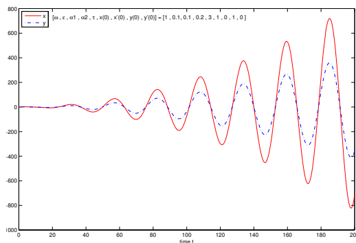
Fig. 2. Plots of x = x_0 + x_1 and y = y_0 + y_1 for [\omega, \varepsilon, \alpha_1, \alpha_2, \tau, x(0), \dot{x}(0), y(0), \dot{y}(0)] = [1, 0.1, 0.1, 0.2, 3, 1, 0, 1, 0] .
