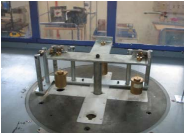
Fig.3. Calibration rig mounted on the floor of the wind tunnel test section
