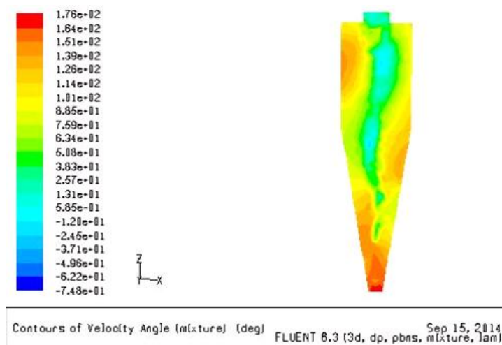
Fig. 10 Velocity direction within the hydrocyclone
