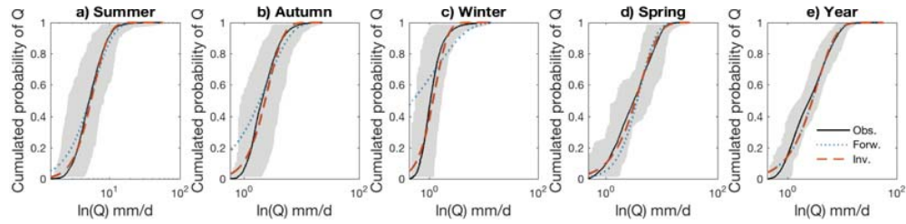
Fig. 3 Cdfs for the linear model in GRO
