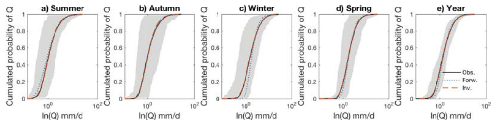
Fig. 5 Cdfs for the nonlinear model in MUW
