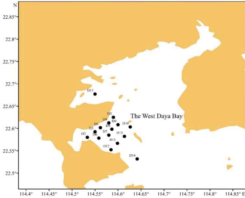
Fig. 1 Survey distribution in the West Daya Bay
