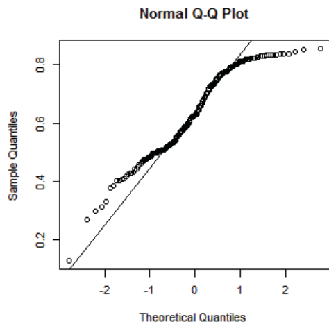
Fig. 2 Quantile-quantile plots of GLM
