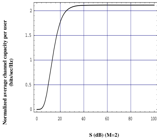
Fig. 1 Normalized average channel capacity (in bits/sec/Hz) per user for a DS/FFH-CDMA cellular system under power and rate adaptation against the the signal-to-noise ratio (SNR) \Gamma (expressed in dB) in a Rayleigh fading environment for M=2 .
