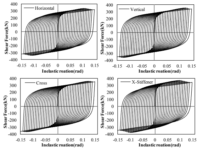
Fig. 13 Effect of stiffener on hysteretic loops
