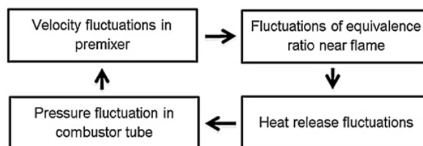
Fig. 1 Mechanism of combustion instabilities
