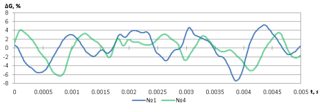
Fig. 9 Mass flow fluctuations through 2 passages
