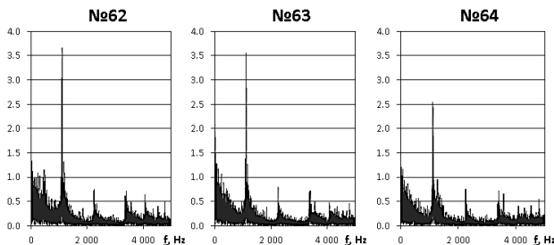
Fig. 3 Spectra of microphones signal
