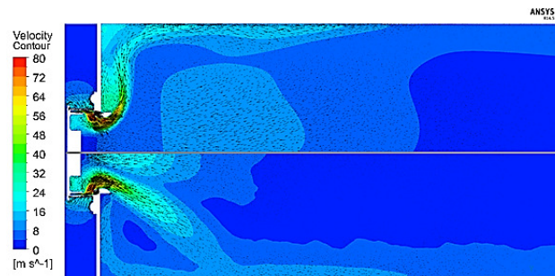
Fig. 11 Comparison of steady (top) and time-averaged (bottom) velocity profiles
