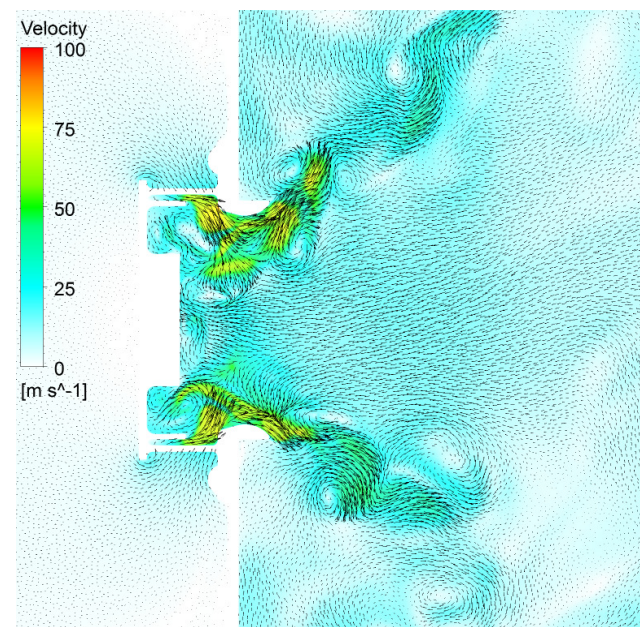
Fig. 8 Strong vortical structures, generated by the swirler
