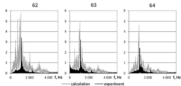
Fig. 10 Spectrums of filtered signals
