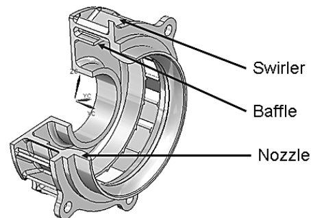
Fig. 4 Studied swirler
