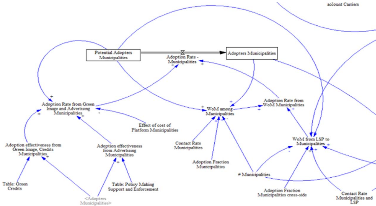
Fig. 1 Municipalities Sub-Model
