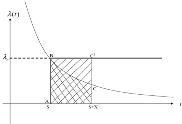
Fig. 1 The testing reliability and the operational reliability (when \lambda(t) to strictly decreasing for t \geq 0 )
