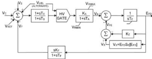
Fig. 2 IEEE type DC1A excitation system model ©IEEE 2005 [7]
