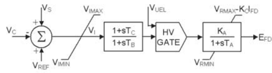
Fig. 3 IEEE type AC4A excitation system model ©IEEE 1991 [4]
