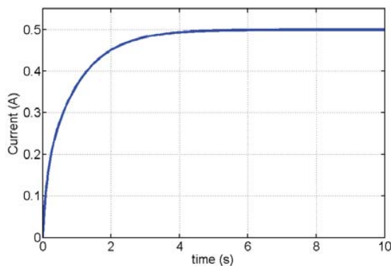
Fig. 7 generator output using DC1A exciter
