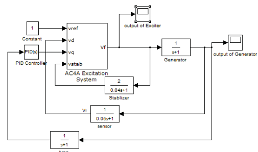
Fig. 5 Software Analysis (SIMULINK based diagram) Using AC4A exciter
