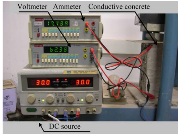
Fig. 2. Measured diagram of the press-electrode method.
