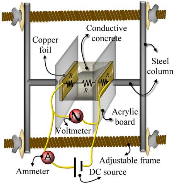
Fig. 1. Structure of the press-electrode method.
