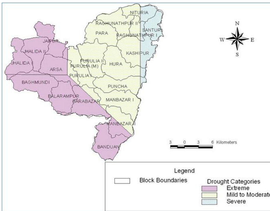
Fig. 5 Study area showing drought severity
