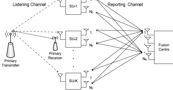
Fig. 1 Cooperative - MIMO reporting system
