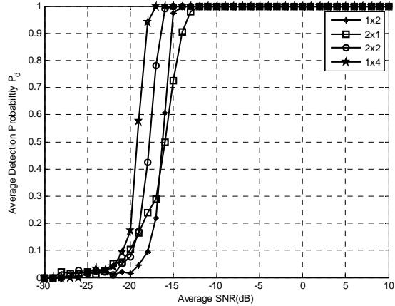
Fig. 4 ZF Multi User
