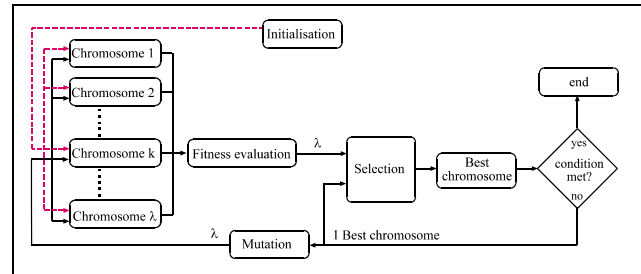
Fig. 3 (1+\lambda) rudimentary evolution strategy
