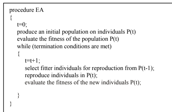
Fig. 1 Classic Evolutionary algorithm
