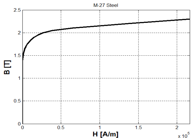
Fig. 5 B = f(H)
