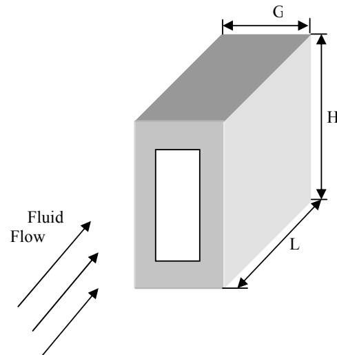
Fig. 2 Computational domain of micro channel heat sink
