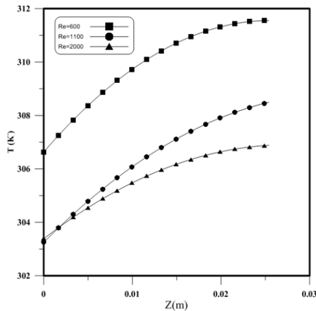
Fig. 4 Variation of Temperature against Z axis in the base of micro-channel
