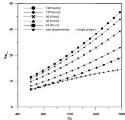
Fig. 3 Variation of Nusult number against Re in the base of micro-channel
