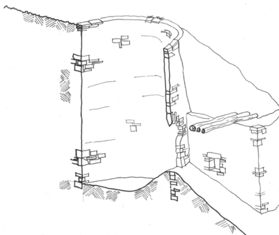
Fig. 1 Sketch of a section through a typical Corsican lime kiln at the Pointe of the Cap Corse
