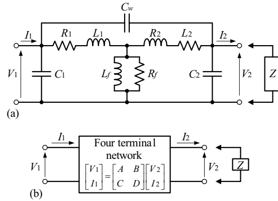
Fig. 6 Equivalent circuit of the transformer.
