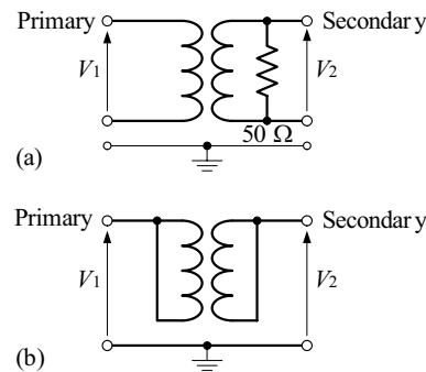
Fig. 3 Measurement method of noise attenuation. (a) Normal mode. (b) Common mode.
