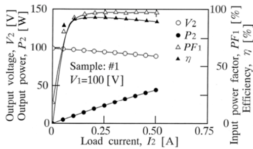
Fig. 2(a) Load characteristics of sample #1.
