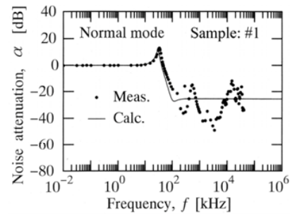
Fig. 7 Normal mode noise attenuation characteristics.
