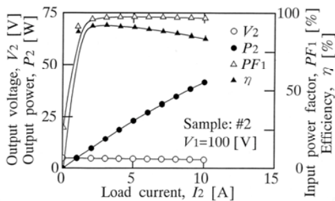
Fig. 2(b) Load characteristics of sample #2.
