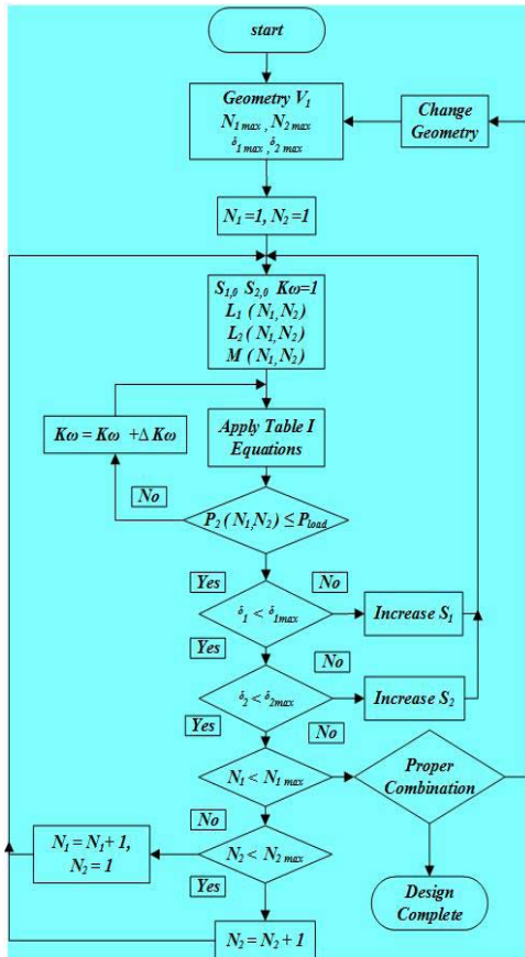
Fig. 1 Flow chart
