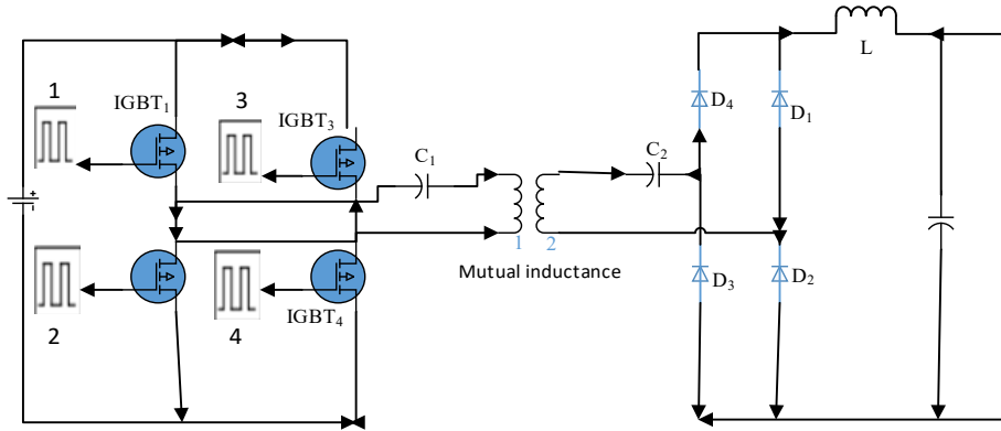
Fig. 8 Simulated circuit
