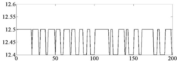
Fig. 5 Cross-section area variation for the secondary for each step (in \text{mm}^2 )
