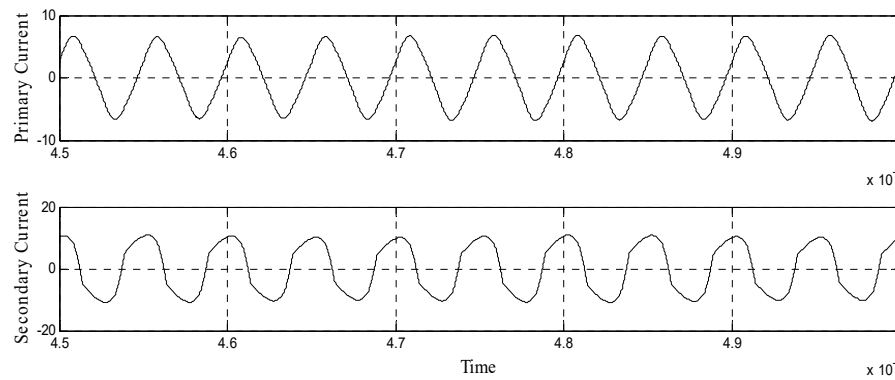
Fig. 10 Primary and secondary currents
