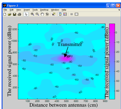
Fig. 4(b) The results of propagation for (9x13 m 2 ) are shown as top view
