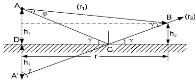
Fig. 1 The two ray model
