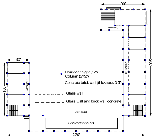
Fig. 2(a) Plan view of experimental building
