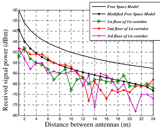
Fig.6 Comparison of modified free space model and experimental data
