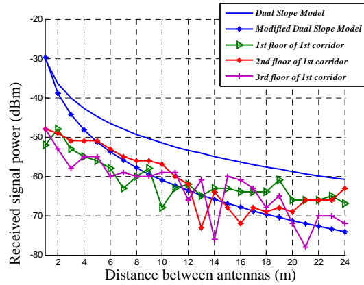
Fig.7 Comparison of modified two ray model and experimental data
