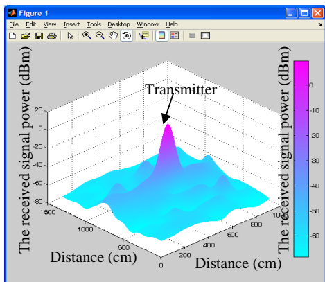
Fig. 4(a) The results of propagation for (9x13 m 2 ) room are shown as 3D
