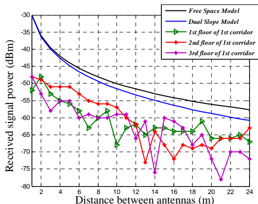
Fig. 5 Two models and experimental data
