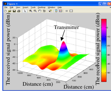
Fig. 3(a) The results of propagation for (4x9 m 2 ) room are shown as 3D
