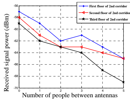
Fig. 8(b) Comparison of modified two ray model and experimental data
