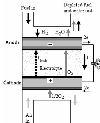
Fig. 5. Principle of a solid oxide fuel cell
