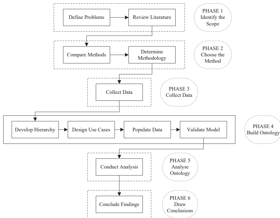
Fig. 1 Research methodology
