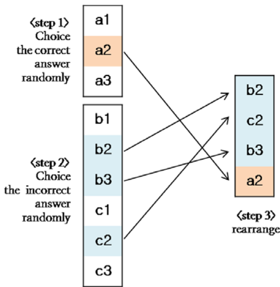
Fig. 3 Creating Examples of Question A
