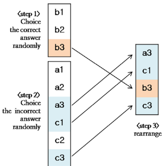
Fig. 4 Creating Examples of Question B
