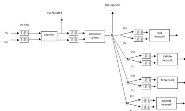
Fig. 3 Queuing network model for this project
