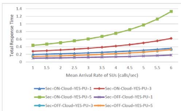
Fig. 9 Total mean response time in scheme B
