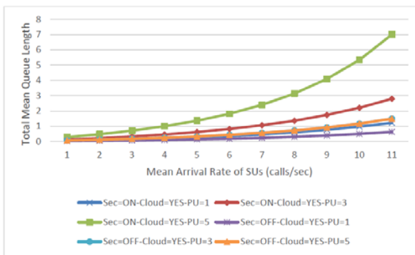
Fig. 10 Total mean queue length in scheme B
