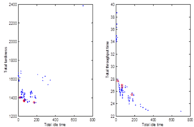
Fig. 4 Pareto optimal set in a three-dimensional space
