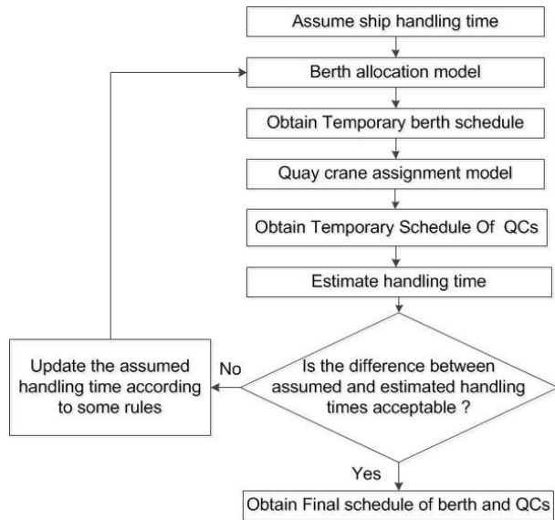
Fig. 6 Flow chart of functional integration with feedback
