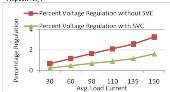
Fig. 10 Voltage Regulation
