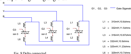
Fig. 9 Delta connected
