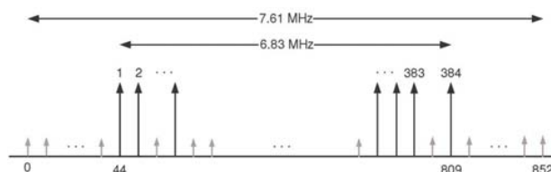
Fig. 1. The P1 symbol in the DVB-T2 system
