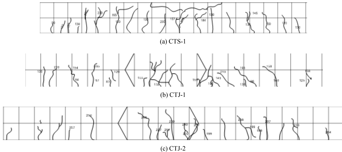
Fig. 17 Crack surface
