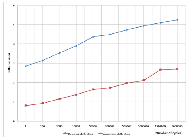
Fig. 15 CTJ-2 deflection
