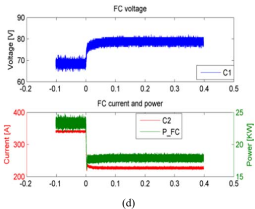
Fig. 2 FC dynamic test results: a) Small load step from small to medium load. b) Medium load step from small to medium load. c) Big load step from high to full load. d) Big load release from full to high load
