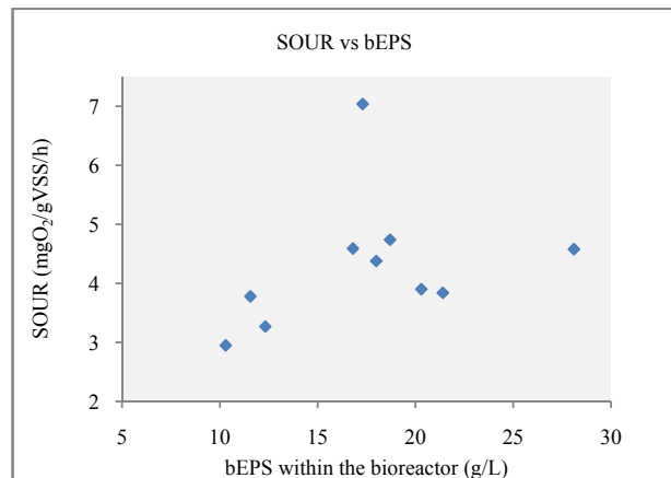
Fig. 4 SOUR vs. bEPS of the CMBR system
