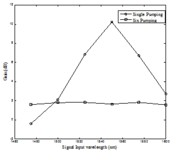
Fig. 2 Variation of Raman gain for single span of Raman fiber length of 10 km
