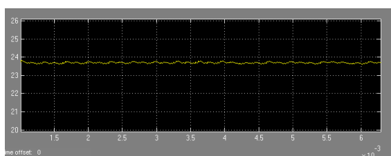
Fig. 18 Results on ripple output voltage for FLC closed loop circuit DC to DC boost converter
