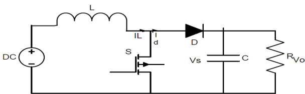
Fig. 2 Basic Circuit of Boost Converter
