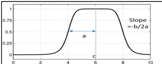
Fig. 7 Generalized Bell Membership Function Shape
