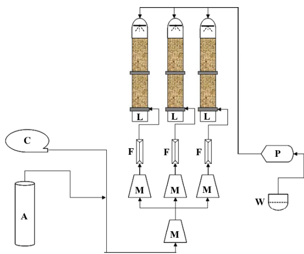
Fig. 2 Flow diagram of biofiltration process (A= \text{NH}_3 gas tank, C= compressed air equipment, F = flow meter, L = Leachate tank, M = mixed air and \text{NH}_3 gas tank, P = peristaltic pump, and W = water tank)
