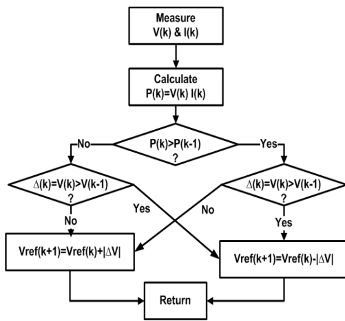
Fig. 10 POMPPT algorithm
