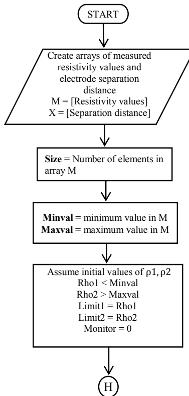
Fig. 4 Data acquisition section of the algorithm
