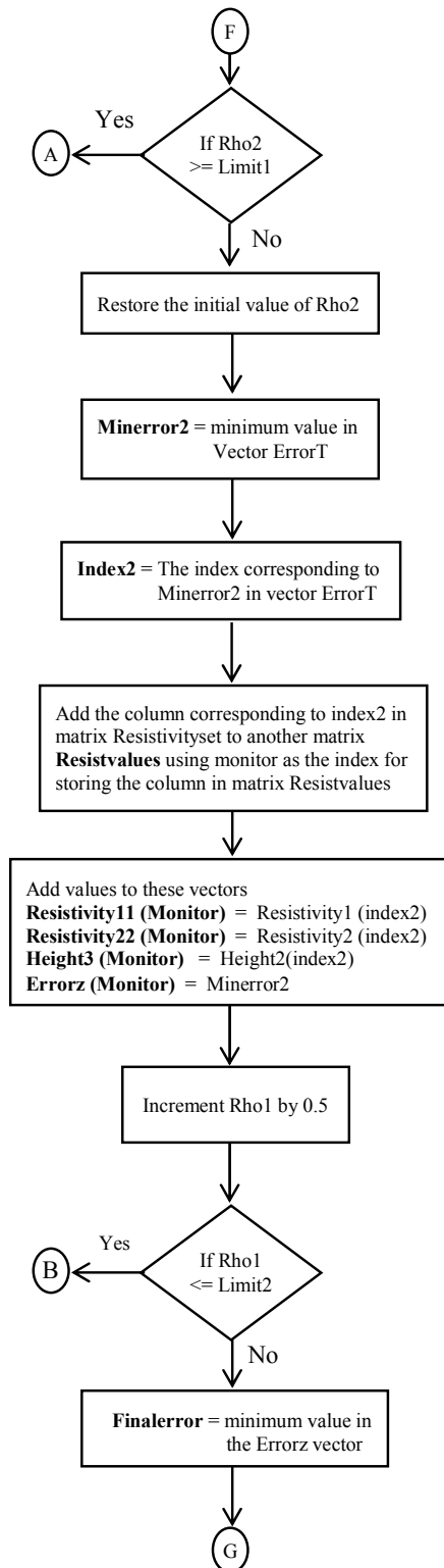
Fig. 7 Algorithm section for evolving the resistivity model
