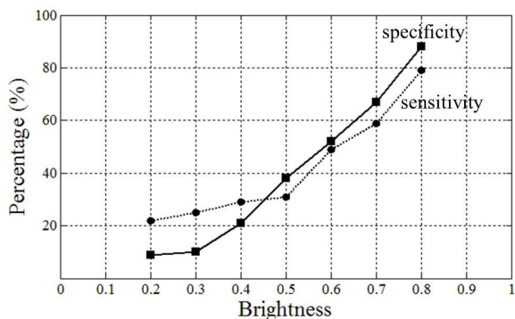
Fig. 1 Capability of detecting bleeding regions as image brightness varies
