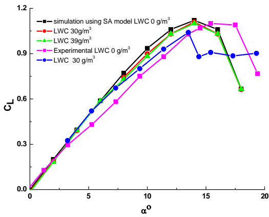
Fig. 10: CL vs. AOA using SA Turbulence Model
