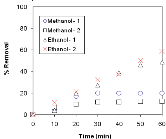
Fig. 6 Percent removal of alcohol over mesoporous siliceous materials
