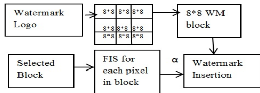
Fig. 9 Watermark Generation process
