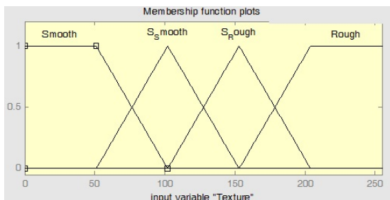
Fig. 3 Texture Fuzzy Membership Function
