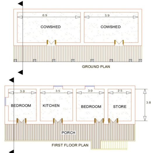
Fig. 3 Typical floor plans of dwellings
