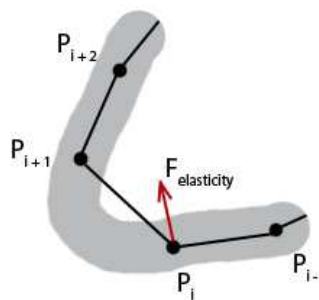
Fig. 2 The elasticity force F_{\text{elasticity}} drags the control point into the object
