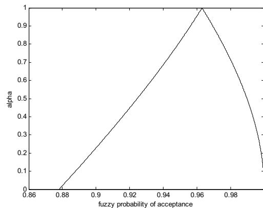
Fig.1 fuzzy probability of acceptance with \tilde{p} = (0, 0.005, 0.01)
