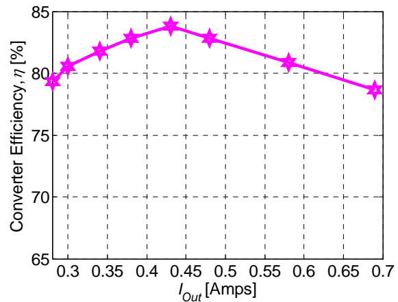
Fig.12 Measured efficiency of the flyback converter circuit with various load resistances
