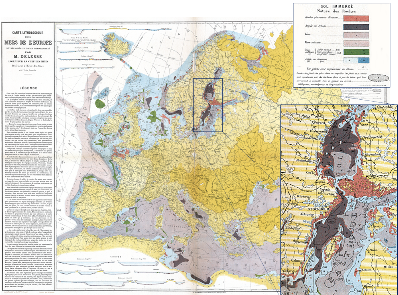
Fig. 2 Lithological map of European seas [32]
