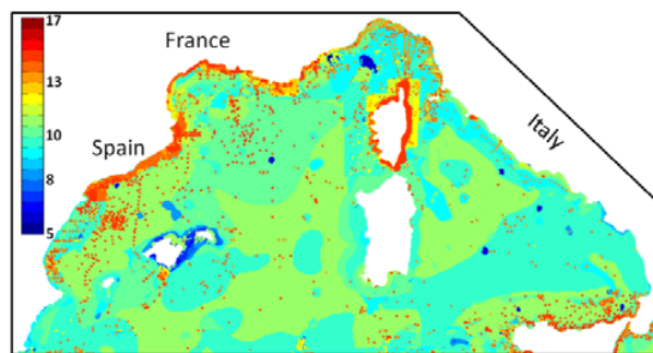
Fig. 7 Map of quality of knowledge rated from zero to 20, for the map to 1:500,000 from the western Mediterranean integrated into the global sediment map
