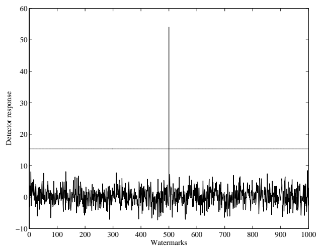
Fig. 8 Response of watermark detector for "Lena"
