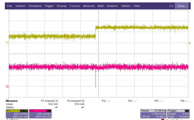
Fig. 7 The output of S&H (top), the input current to the converter (bottom)
