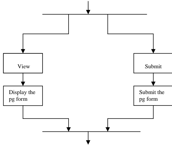
Fig. 3 An Activity Diagram for Postgraduate Student
