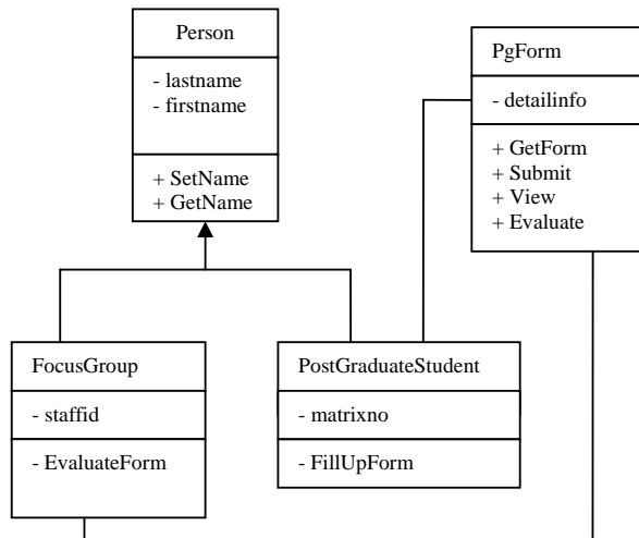
Fig. 4 A Class Diagram for Monitoring System of Postgraduate Student
